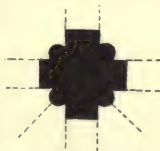
Fig. 283.—Milan. San Babila. Section of pier (XIth Century).
